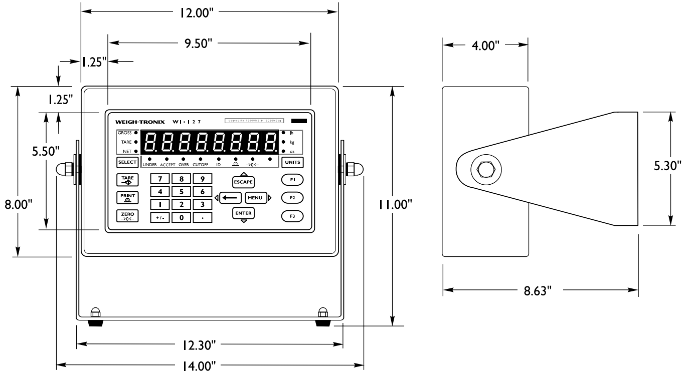
Front view - desk top stand
